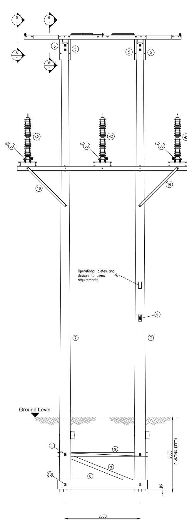
SECTION 1 Scale 1:35
