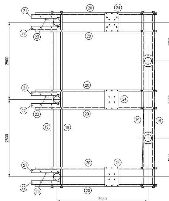
SECTION 3 Scale 1:35
