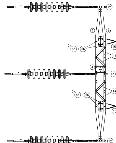
SECTION 4 Scale 1:35
