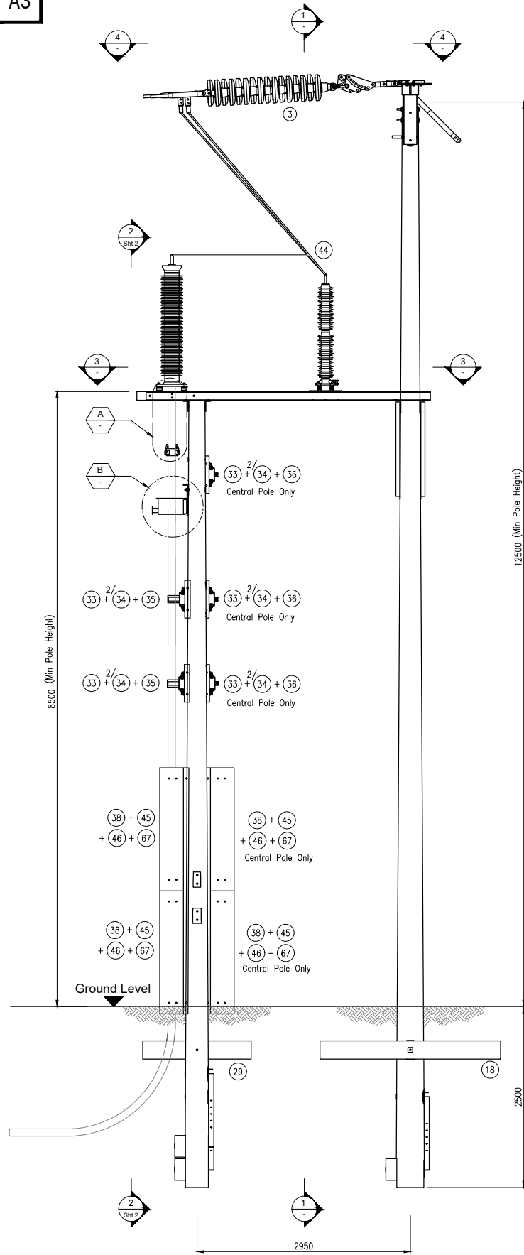
SIDE ELEVATION
